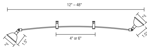
Cable/Twin Rail
